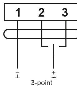
AC/DC 21...27V
